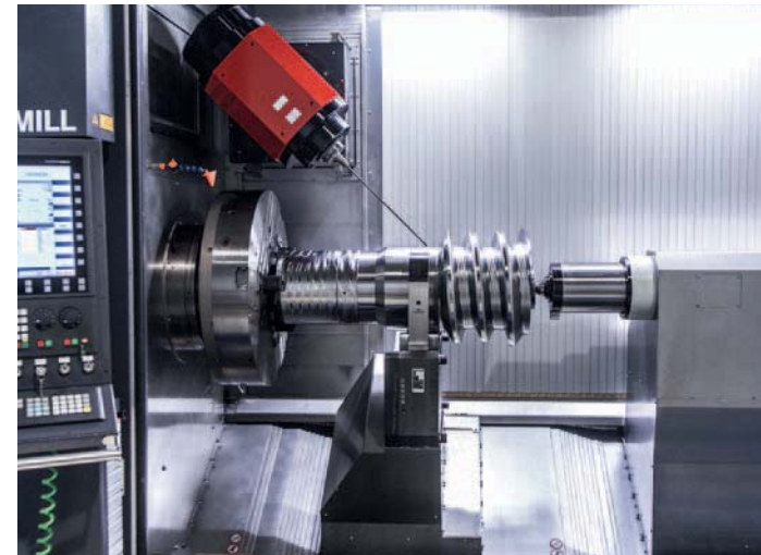
Deep hole drilling for diameters of up to 6 x 500 mm with a maximum of 80 bar
