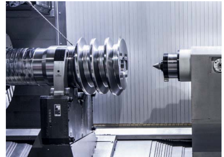
Tailstock: adjustable tailstock (MK6) for a workpiece weight of up to 6 t
