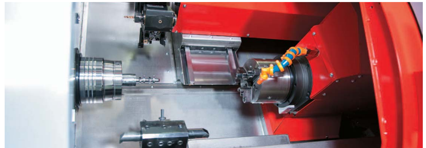
Work area. The generous work area provides space for several tools on both turrets and ensures a continuous chip flow even when few machine technicians are at work. Additional coolant pumps and a sophisticated pipe system clears the chips into the chip conveyor.
