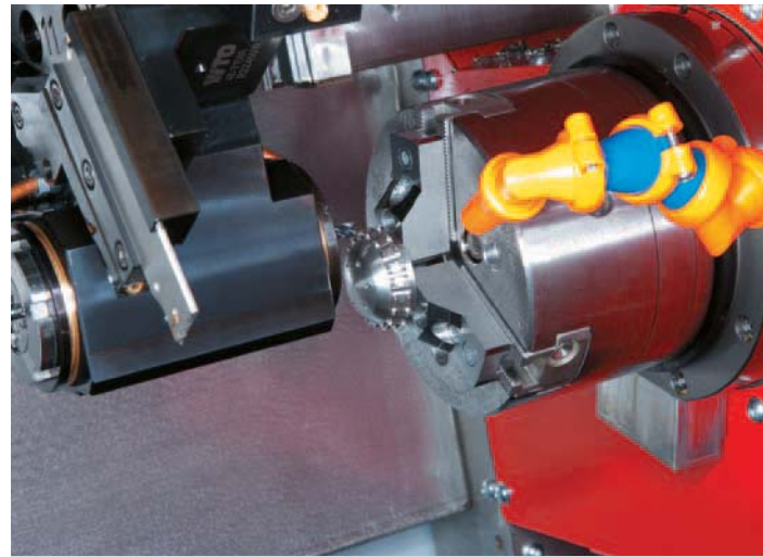
Counter spindle. A 15 kW, water-cooled spindle motor ensures dynamic performance and high levels of precision. The standard machine is equipped with a coolant-fed parts ejector. This places the finished workpieces in the parts catcher and at the same time clears the clamping surface from chips. Additionally, a flexible coolant pipe is mounted above the counter spindle for cleaning.
