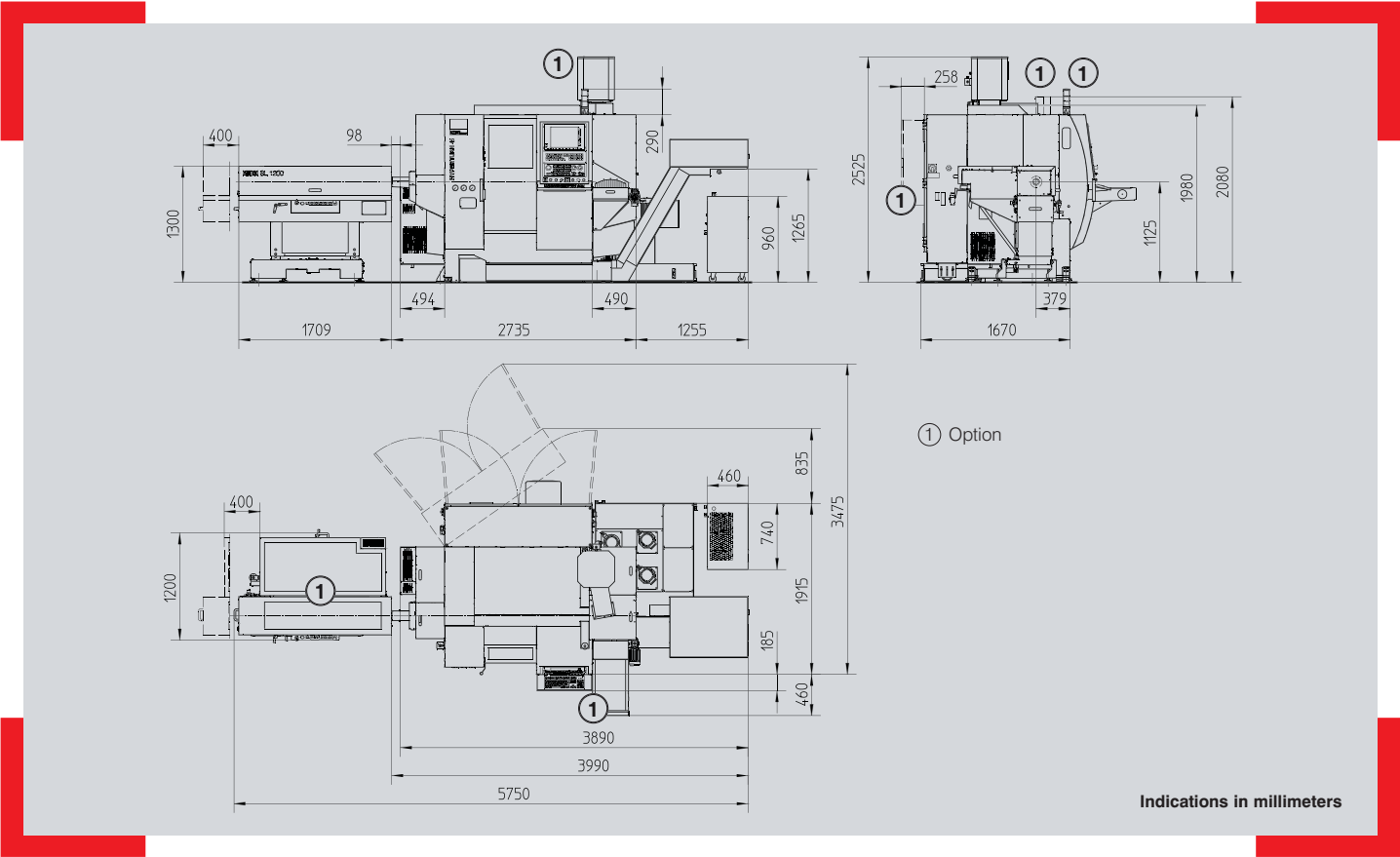
Machine layout EMCO TOP LOAD 8-42/3200
