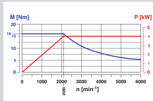
Tool turret - driven tools
