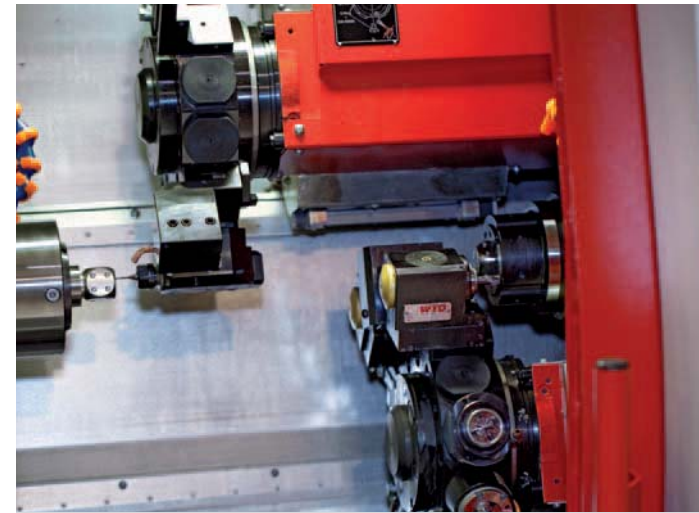
Tool turrets. Rapid 12-fold servo turrets with very short cycle times for standardised VDI25 tools. All stations may accommodate driven tool holders for drilling, milling or thread-cutting operations. The operator may influence the swing speed at any time.
