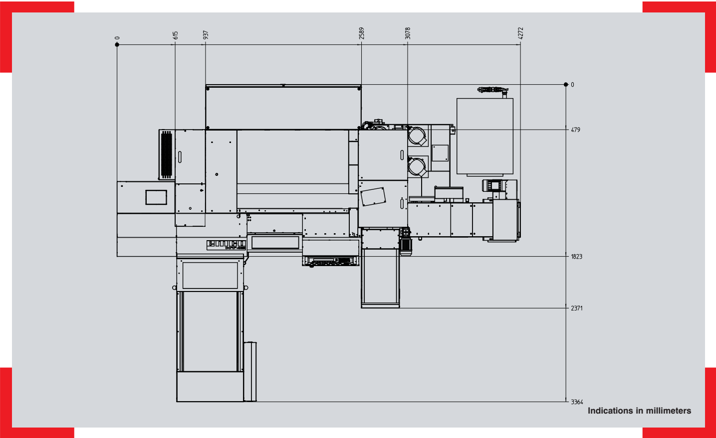
Machine layout HT45 with chip conveyor
