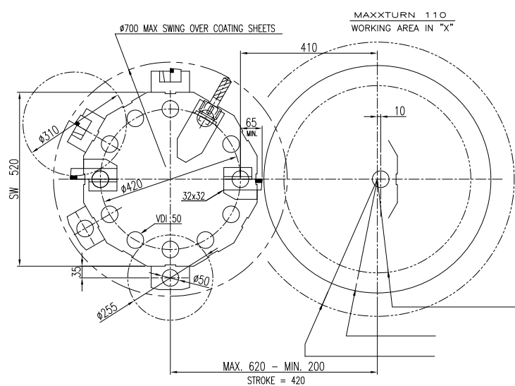
TAILSTOCK WITH QUILL CM5
