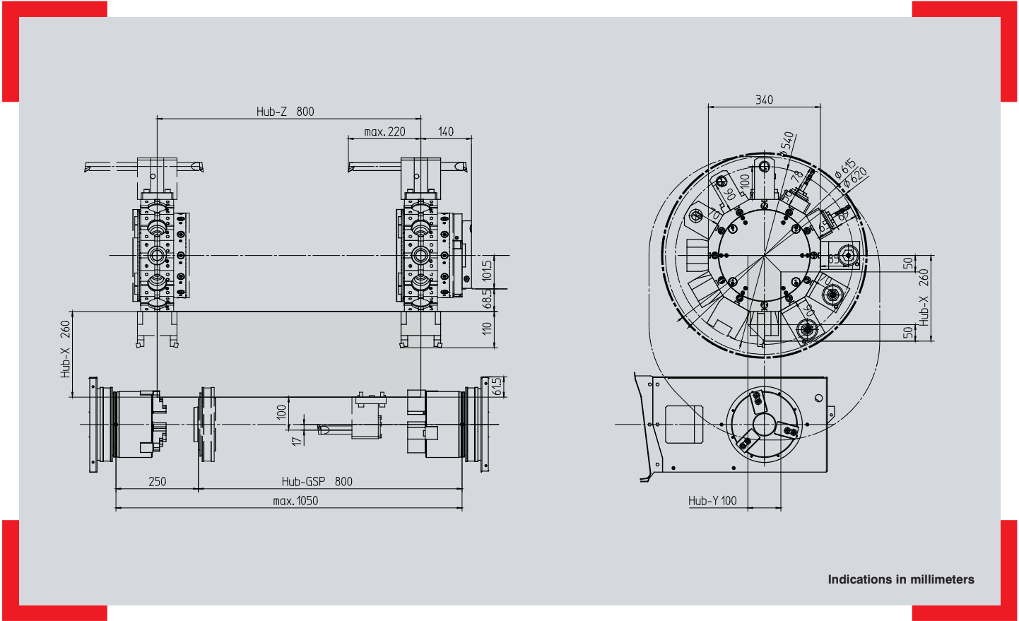
Machine layout Maxxturn 65-1000
