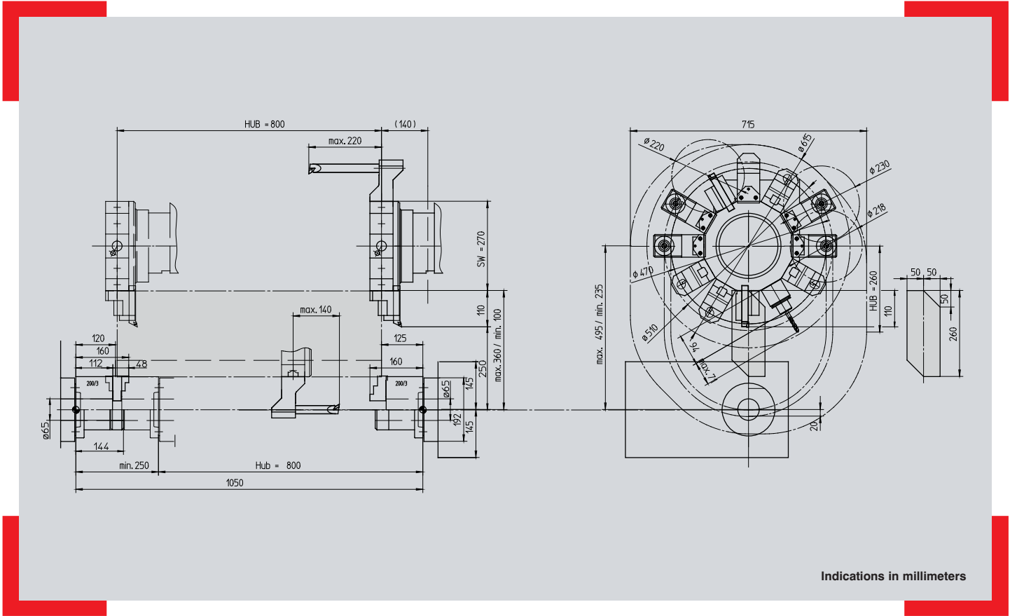
Workspace Maxxturn 65-1000 with VDI40
