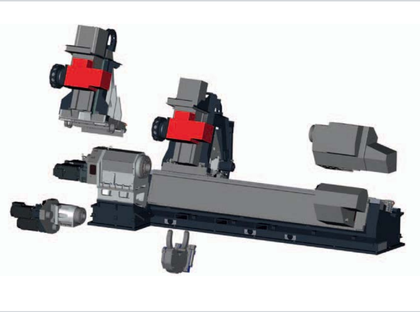
MT3200 – Modular system
